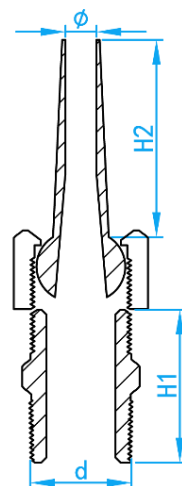
CROSS SECTIONAL VIEW
