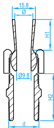
CROSS SECTIONAL VIEW
